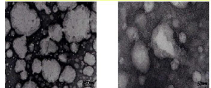
Dispersion pattern comparison between general emulsion (left) and nanosol (right) particles
